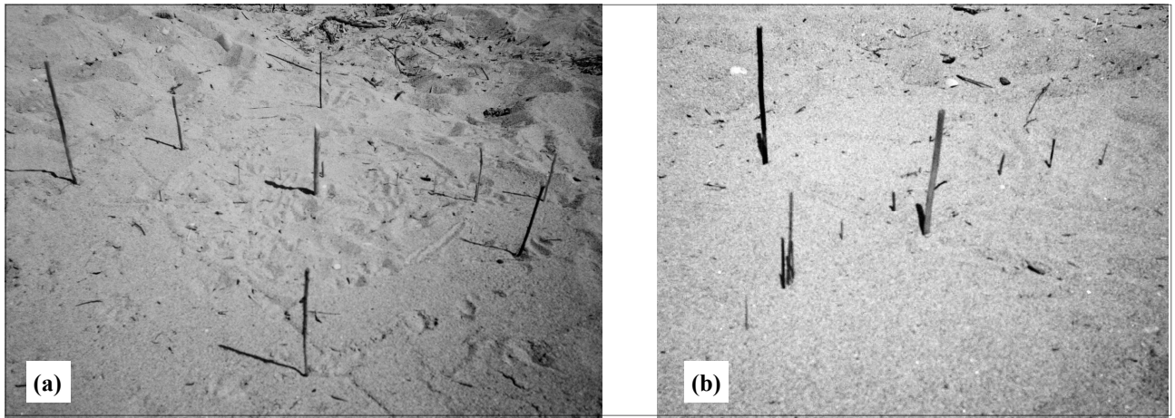
Fig. 6. An example of an exercise using the method of equal altitudes. On a sandy beach shore with lots of tree sticks washed ashore, nature provides right at hand most of the equipment for a rough and ready tryout of this method of determining the meridian. The tall central stick is the gnomon. Observations taken c.7 June 1992 at Southampton by Lake Huron, Ontario, Canada, latitude \phi \approx 44^{\circ}30' N . Photo taken the next day.
