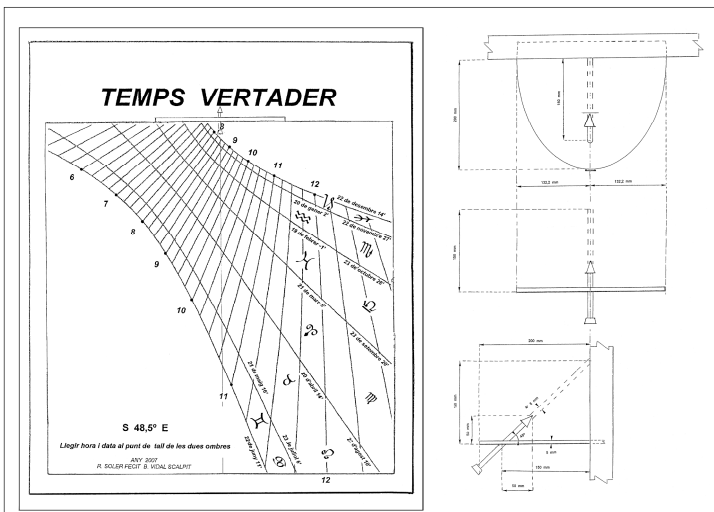
Fig. 8. Drawing of the SE face (left) and (right) the design for the gnomons (all faces).
