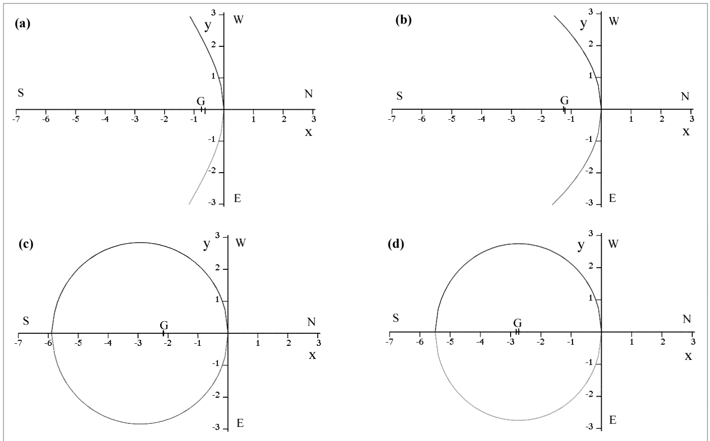
Fig. 3. Shadow curves described by the tip or apex of a shadow cast on a horizontal surface by a vertical gnomon with its base at G. The origin (0,0) point occurs at solar noon. The unit of measurement on the X and Y axes is the vertical height of the gnomon rod above the horizontal surface (TG in Fig. 1).
