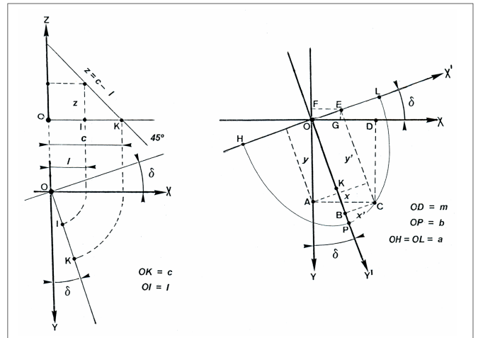
Fig. 7. Coordinate systems for the parametric equations of the gnomons.
