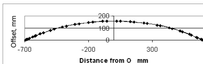
Sunrise marker offsets on date scale (for 51.33° N)
