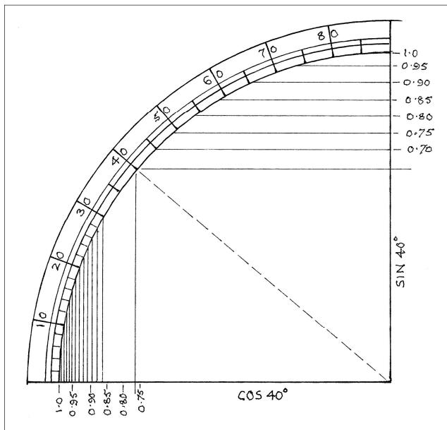
Fig. 21. The principle of the sine/cosine quadrant.
