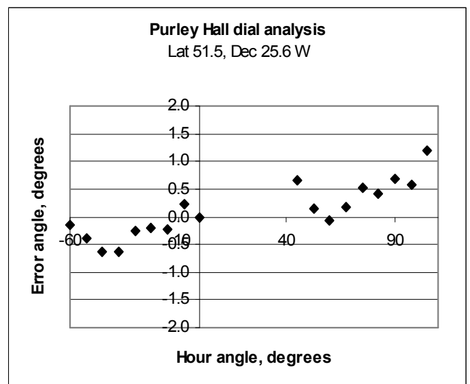
Fig. 11. Error analysis of the hourlines on the Purley Hall dial, for a design latitude of 51.5° N and a best-fit declination of 25.6° W. The lines from the central panel have been omitted.
