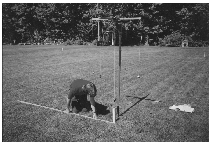
Fig. 4. A reconstruction of the Roman groma surveying instrument. Surmounted on the central pole is a swivelling cross-piece with four plumb-lines for sighting a pair of lines at right angles. The method of equal altitudes was a way to align these lines with the four cardinal directions.
