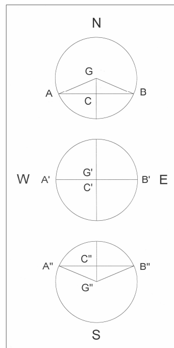
Fig. 2. The method of equal altitudes: possible locations of the line segment BA (indicating E-W) and its midpoint C with respect to the base of the gnomon at G: (top) BA to the south of the gnomon at G, (middle) B'A' coincident at C' with the gnomon's base at G and (bottom) B''A'' to the north of the gnomon at G''.
