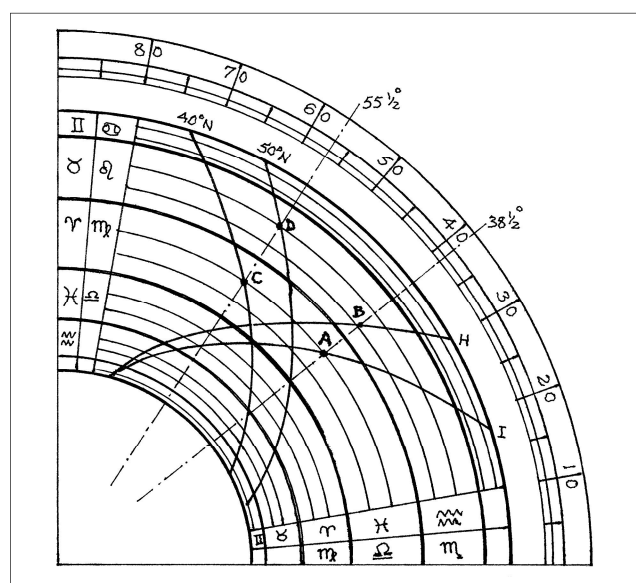
Fig. 23. The use of the arcs of the signs, midday altitude and Qibla.
